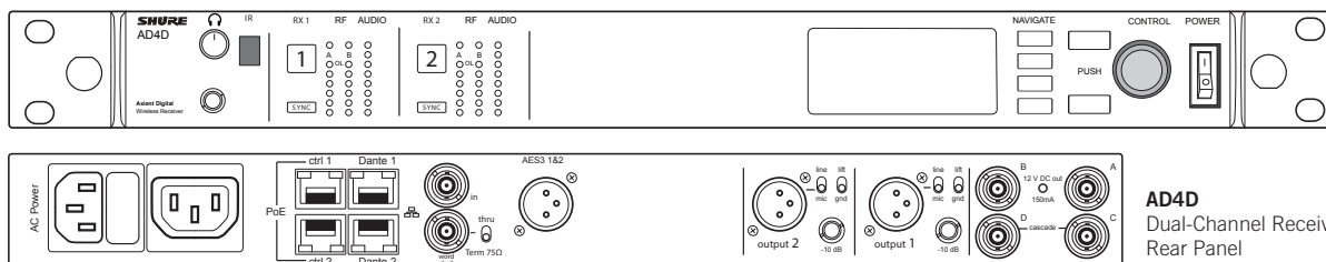
AD4D Dual-Channel Receiver Front Panel
